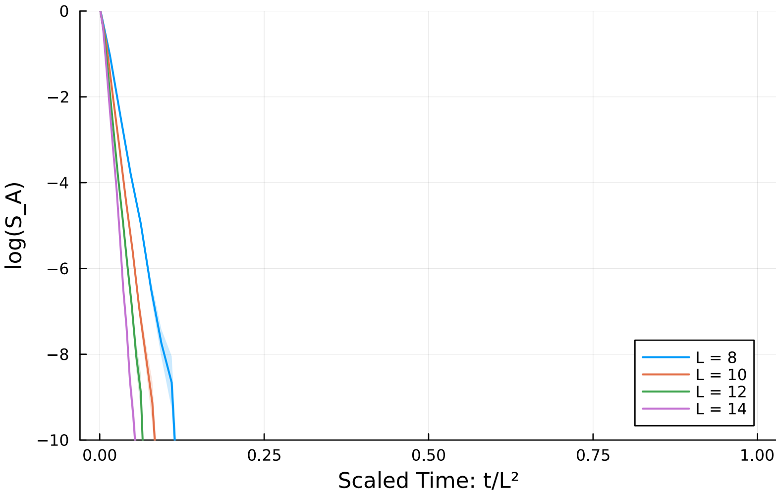
Scaled Log Entropy Evolution ( p = 0.816667 )
